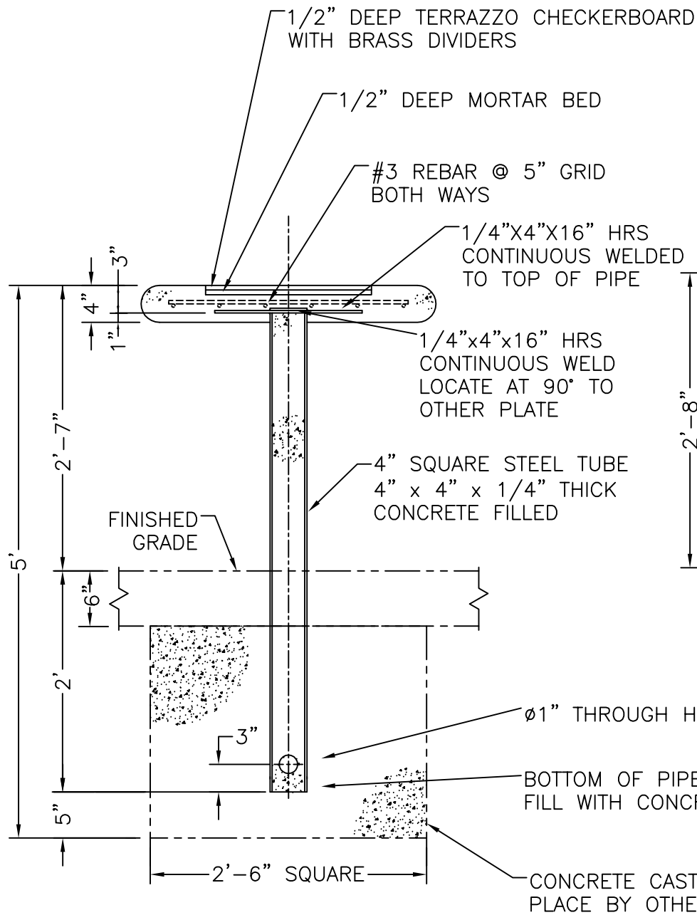
ELEVATION - FULL SECTION
